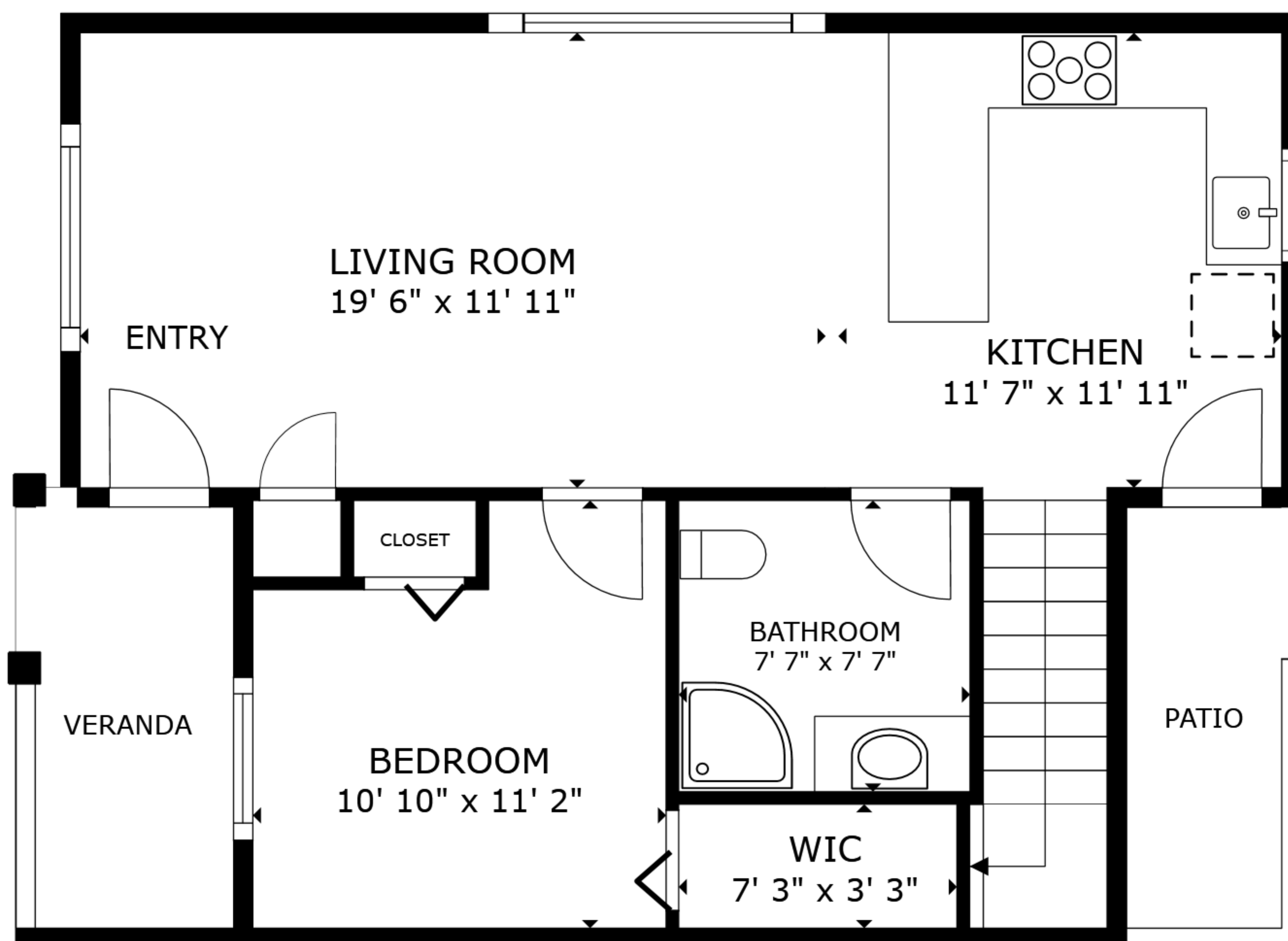
FLOOR 1
