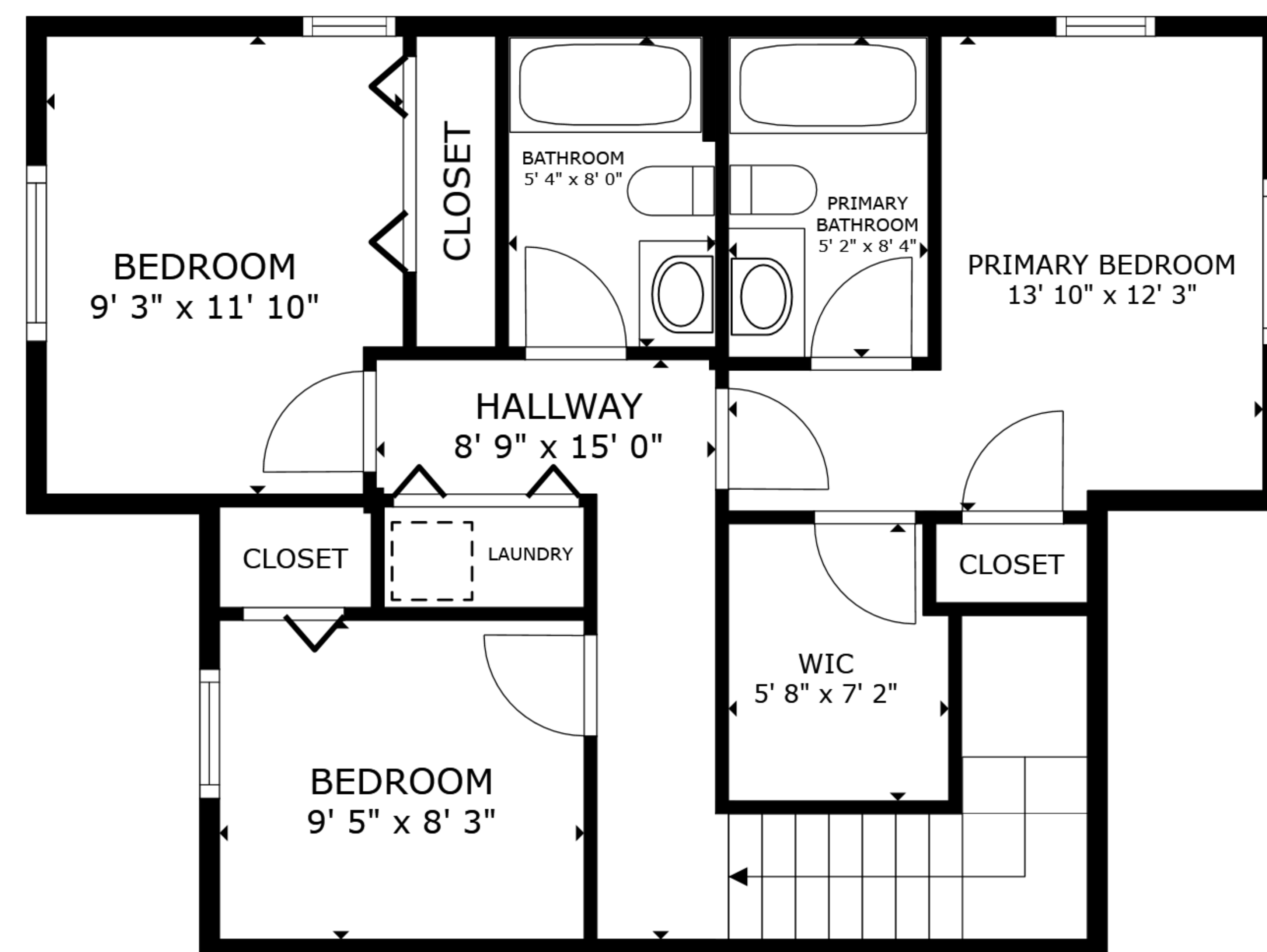
FLOOR 2
